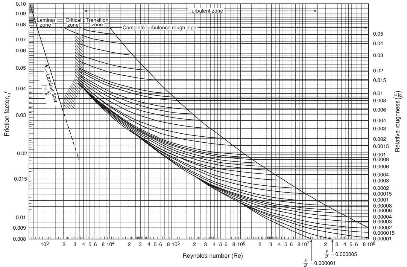
FIGURE A.23.4.4.7.2 Moody Diagram.
