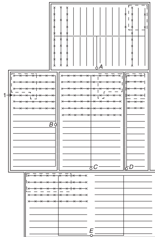
FIGURE A.23.4.1(a) Example of Hydraulically Most Demanding Area.
