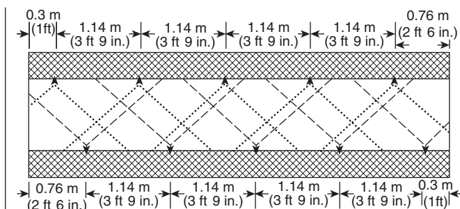
FIGURE A.22.7.1.10(a) Nozzle Layout for Typical Vault. [40:Figure A.6.5.6.6(a)]
