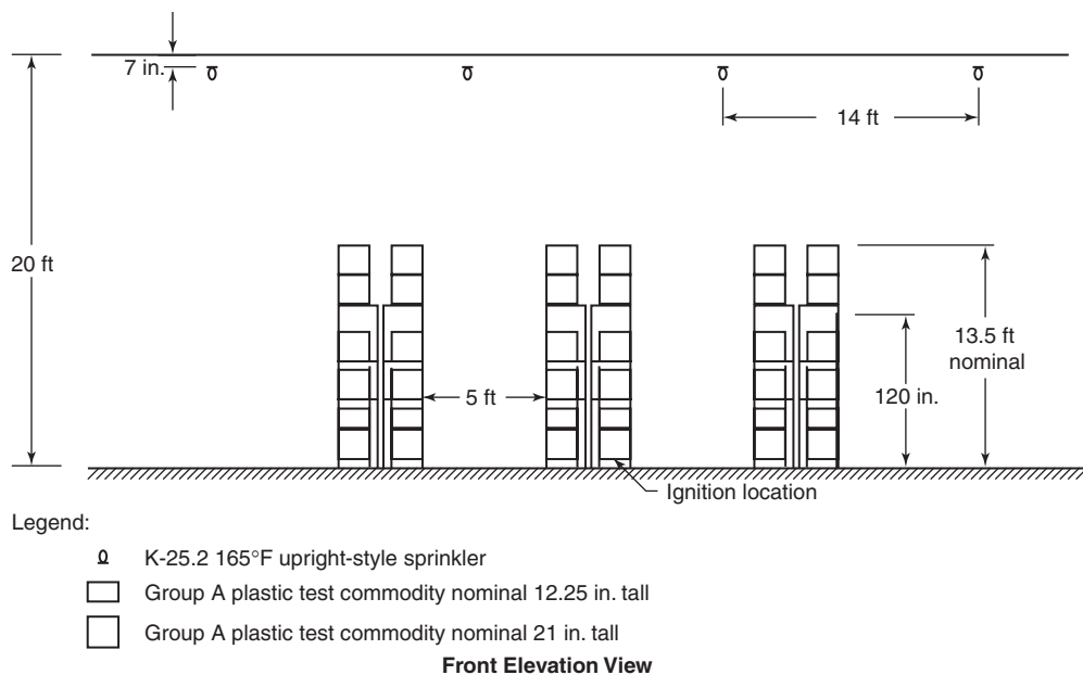
FIGURE A.20.3(d) Fire Test A4.
